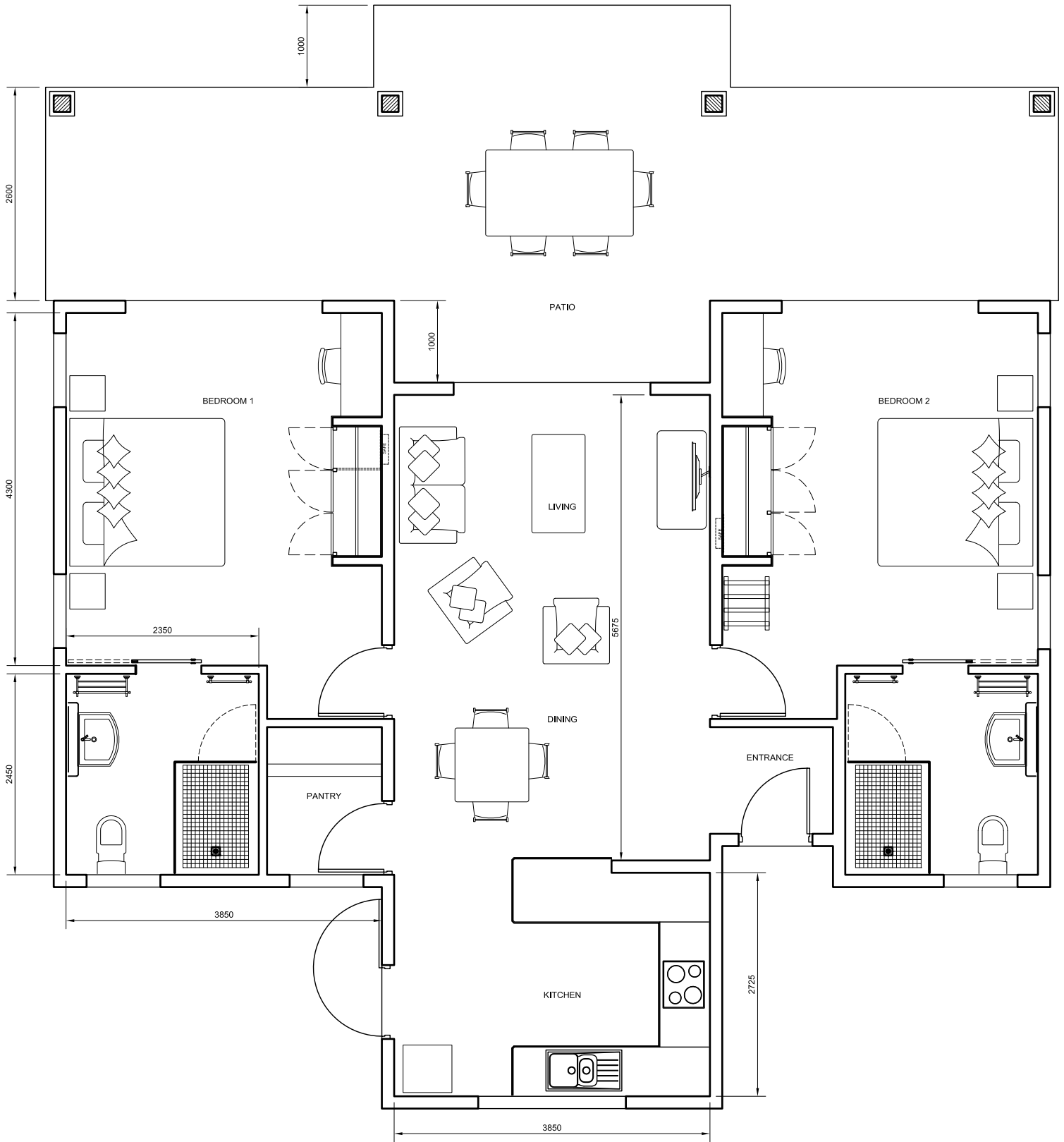
BRL: VILLA LAYOUT. 124Sqm
