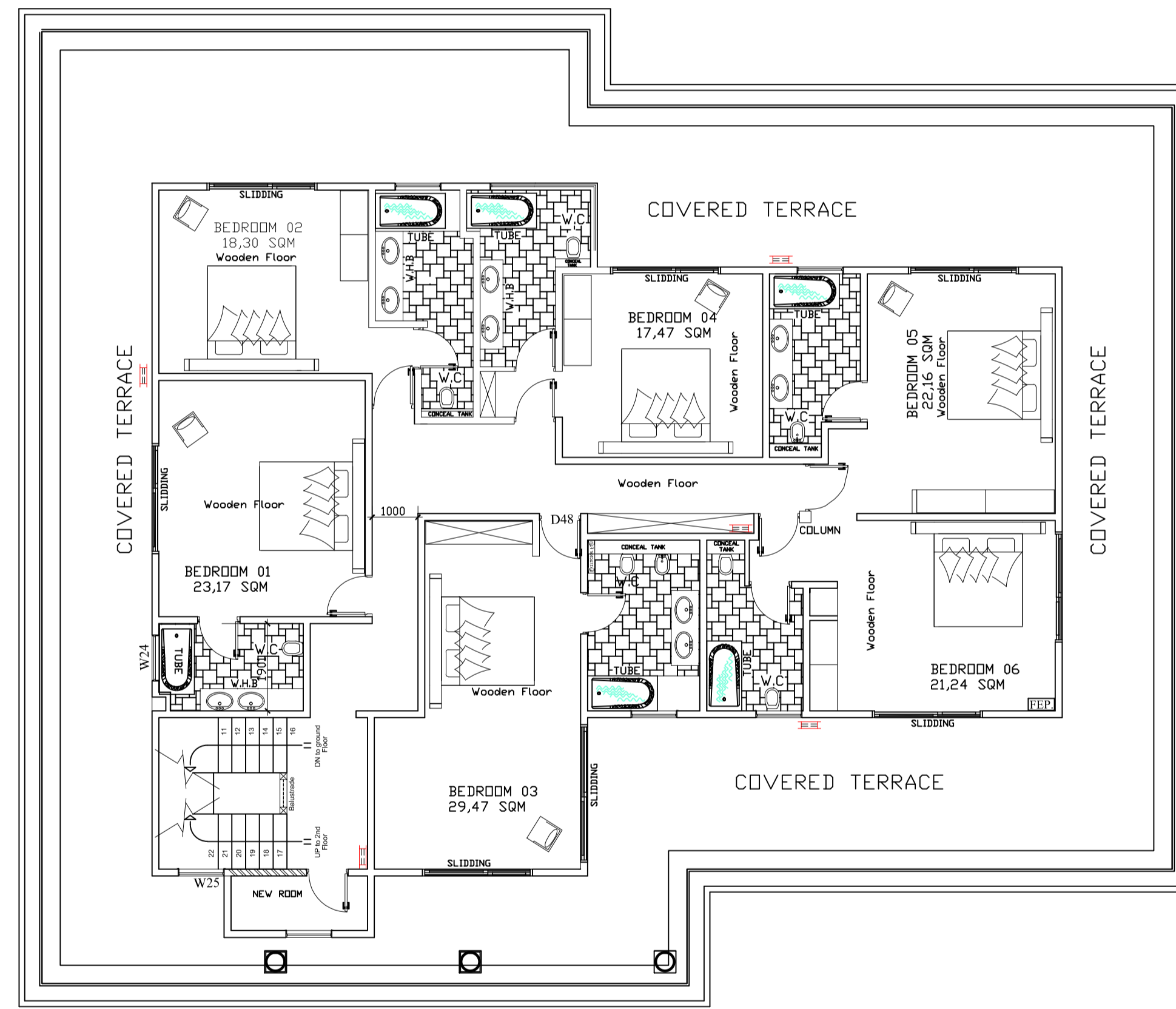
FIRST & SECOND FLOOR LAYOUT PLAN
